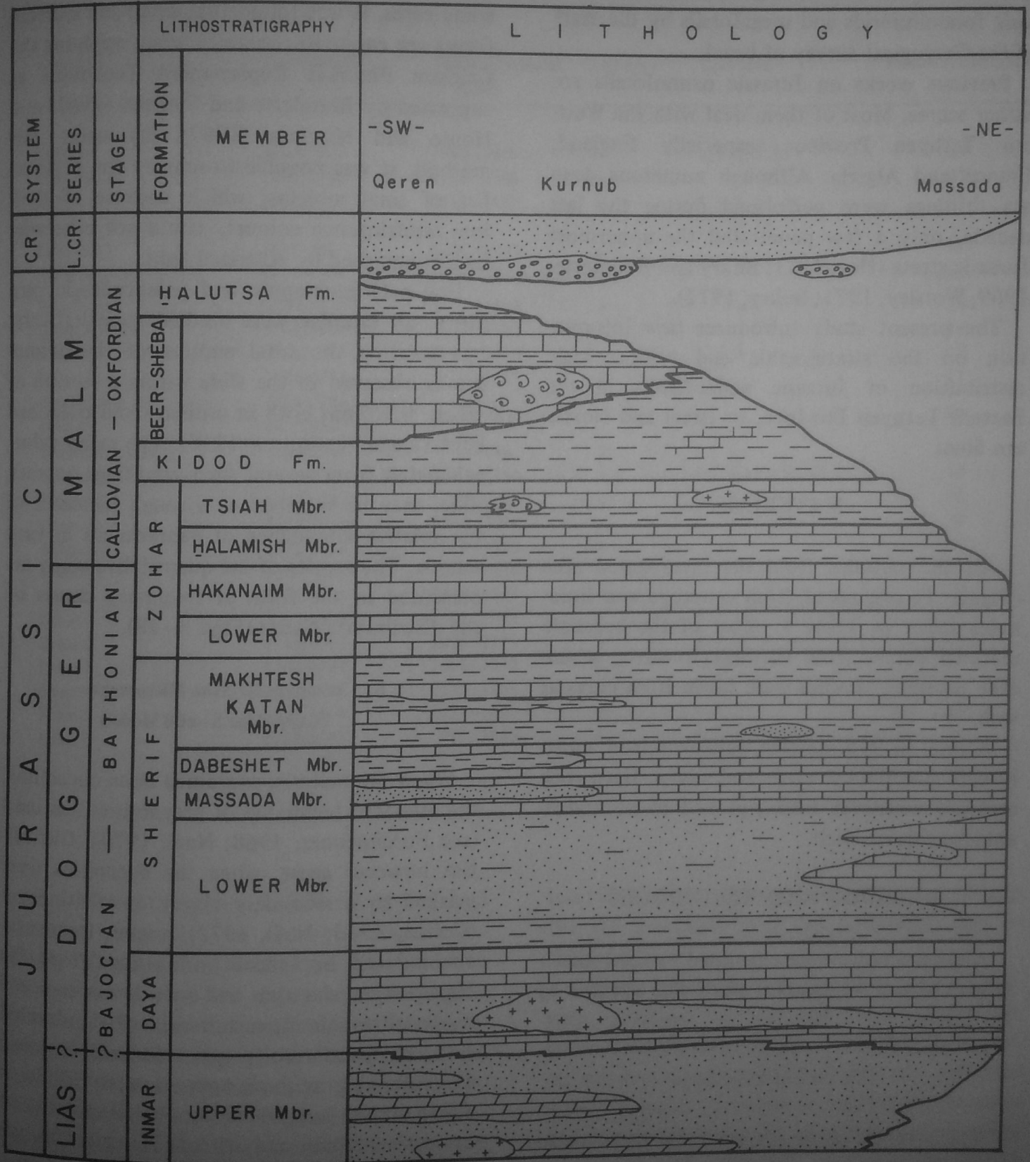
Figure 2: Schematic composite columnar section of the Middle-Upper Jurassic, Southern Israel (after Goldberg, 1970) (legend: p. 30).
